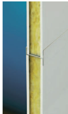
Wall panels joined by H channels. Detail of the glass-wool insulation. Unión de paneles con perfiles en H". Detalle con aislante de fibra de vidrio.
